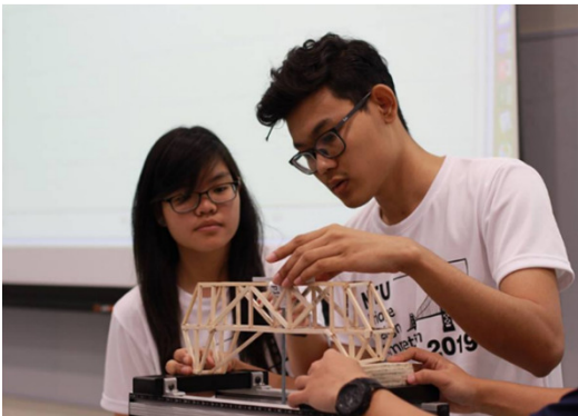
Set-up bridge model on load testing machine
