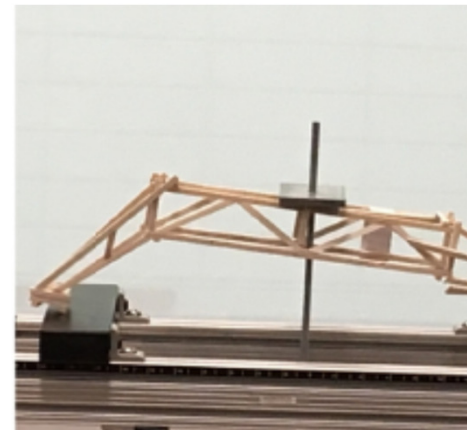
Bridge fail after load testing
