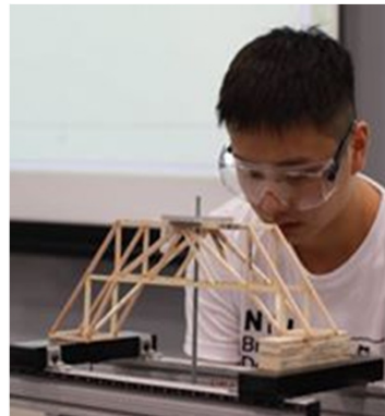
Team member applying load to bridge model
